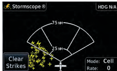
Figure 11-51 Stormscope 360° and Arc Display Views
