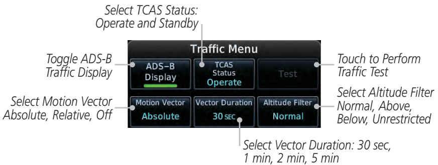
Figure 9-11 ADS-B Traffic Menu
