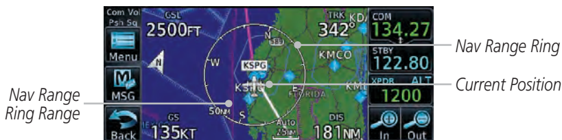
Figure 8-19 Nav Range Ring
