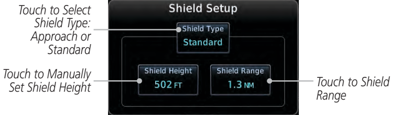
Figure 9-35 TCAD 9900BX Shield Setup for En Route, Standard, and Terminal
