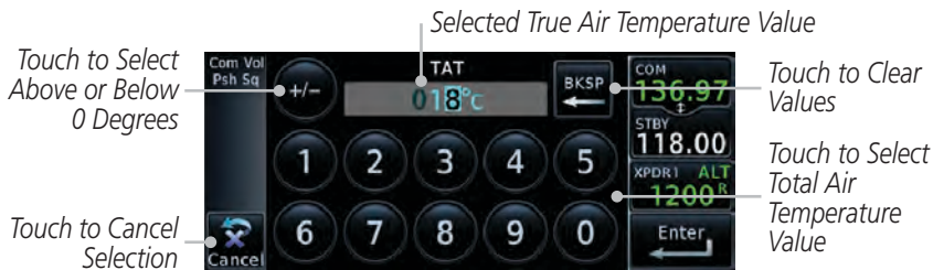
Figure 14-44 Select Total Air Temperature Value
