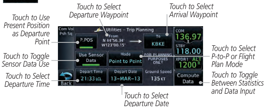
Figure 14-15 Utility Trip Planning Page To Edit Input Data (Point-To-Point Mode) -Sensor Data Used
