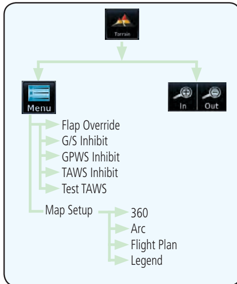
Figure 10-39 TAWS-A Page Functional Diagram
